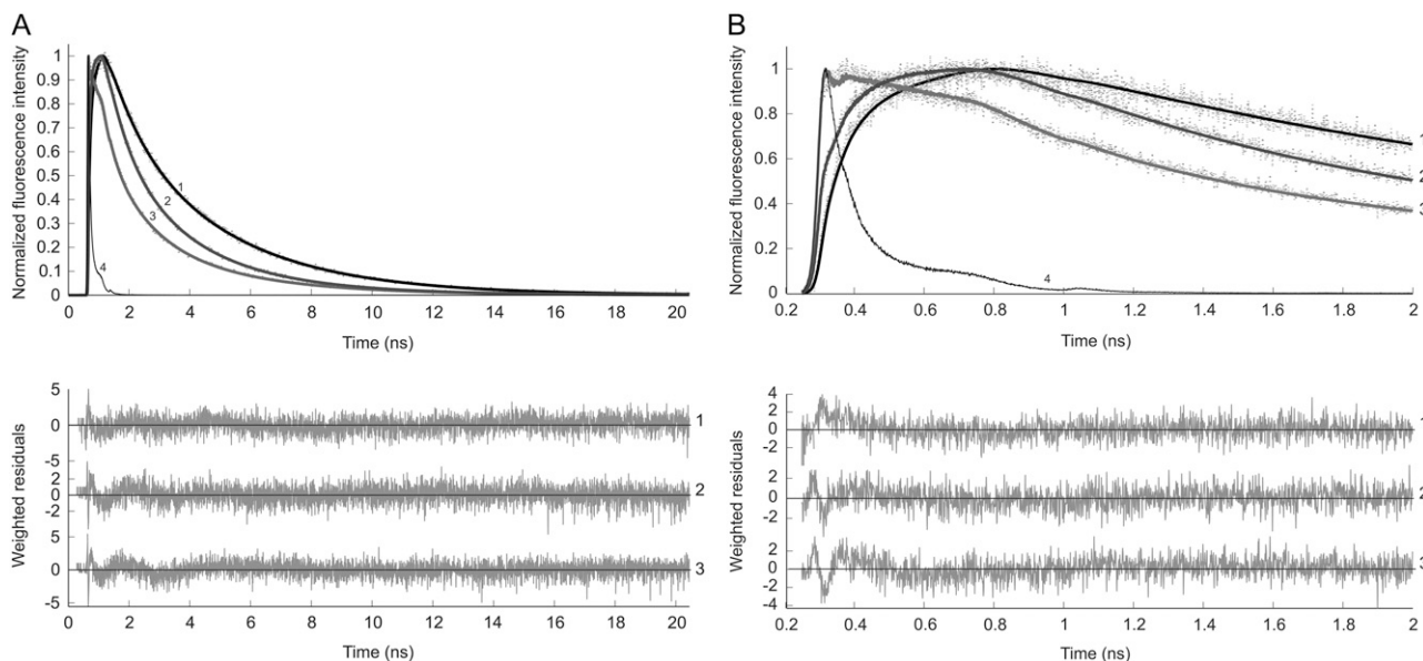
FIGURE 1 Normalized experimental (dotted line) and fitted (solid line) fluorescence decay curves of ECFP (curve 1), YC3.60 in absence of \text{Ca}^{2+} (curve 2), YC3.60 in presence of \text{Ca}^{2+} (curve 3) and the reference compound xanthione in ethanol (curve 4). The excitation wavelength was 400 nm and the detection wavelength of ECFP emission was 480 nm. In A the data are presented with a time scale of 5 ps/channel, whereas this is 1 ps/channel in B, in which only the first 2 ns are shown. The experimental data taken at both time scales are globally analyzed using a multiexponential model with amplitudes \alpha_i and lifetimes \tau_i as adjustable parameters for obtaining an optimal fit. In case of ECFP a bi-exponential decay model with lifetimes 0.97 ns and 3.57 ns was sufficient. The long 3.57-ns lifetime was fixed in the tri-exponential decay model of YC3.60. All recovered parameters ( \alpha , \tau ) are collected in Table 1 (case 1). Weighted residuals belonging to each fitted curve are presented in the bottom panels. Global \chi^2 values are, respectively, for ECFP 1.11, for YC3.60 in absence of \text{Ca}^{2+} 1.14, and for YC3.60 in presence of \text{Ca}^{2+} 1.15.
